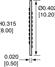
WASHER
