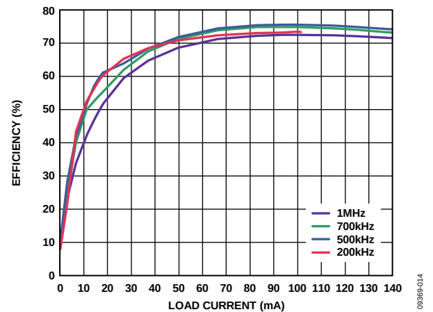
Figure 14. Typical Efficiency at Various Switching Frequencies with Coilcraft Transformer, 5 V Input to 15 V Output
