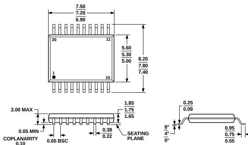
Figure 49. 20-Lead Shrink Small Outline Package [SSOP] (RS-20) Dimensions shown in millimeters
