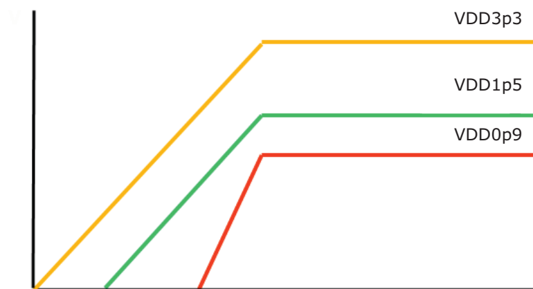
Figure 11-12. Power Sequencing Guideline
