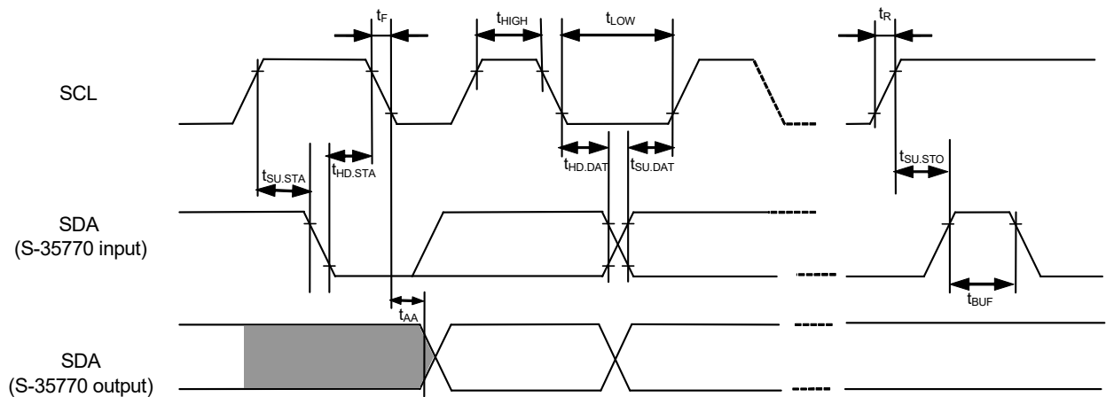
Figure 8 Bus Timing
