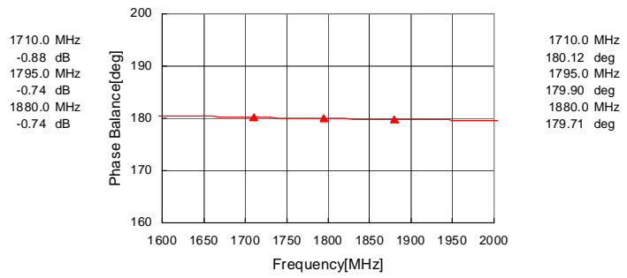
Phase Balance
