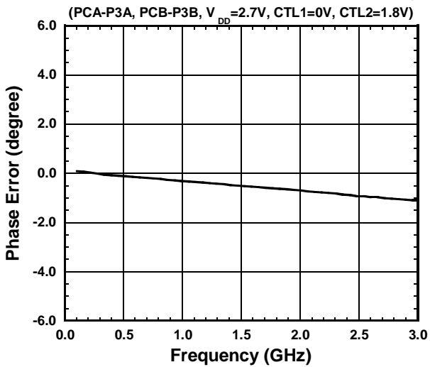
PC-P3 Phase Error vs. Frequency
