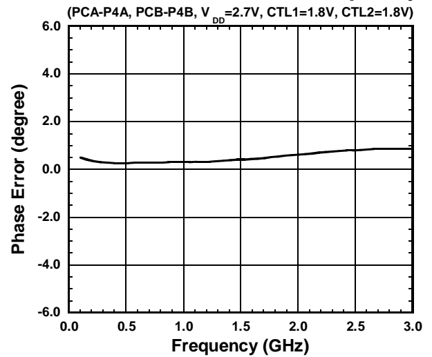
PC-P4 Phase Error vs. Frequency
