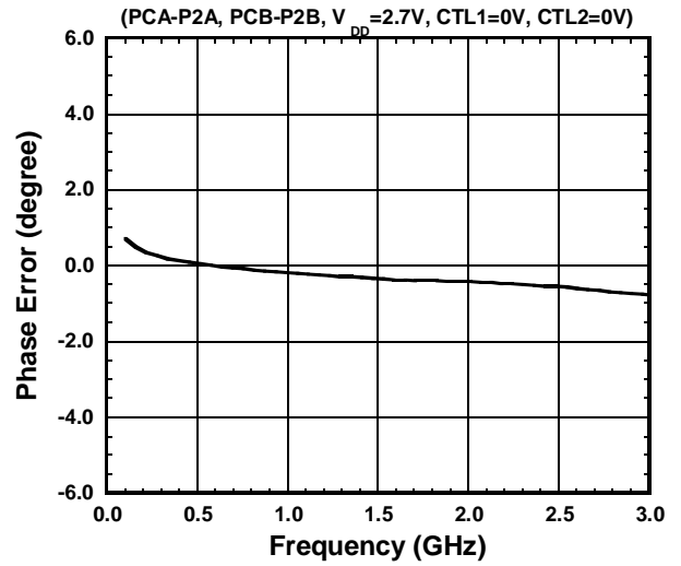
PC-P2 Phase Error vs. Frequency
