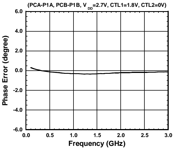
PC-P1 Phase Error vs. Frequency
