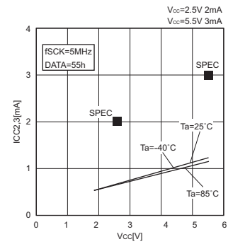
Fig.14 Current consumption at WRITE operation ICC_{1,2,3}(WRITE,PAGEWRITE,WRSR,f_{SCK}=5MHz) BR25L010-W,BR25L020-W,BR25L040-W
