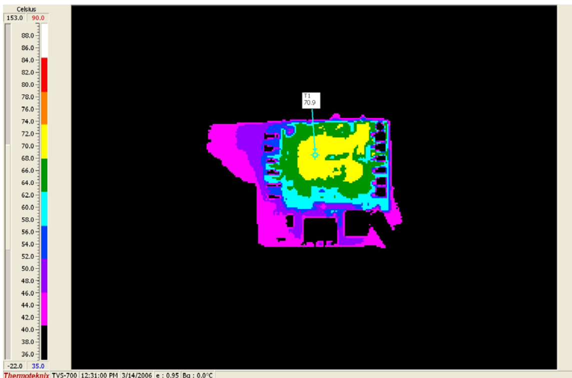
Figure 7. Temp Data (48Vin, 5A, 100LFM airflow – front)
