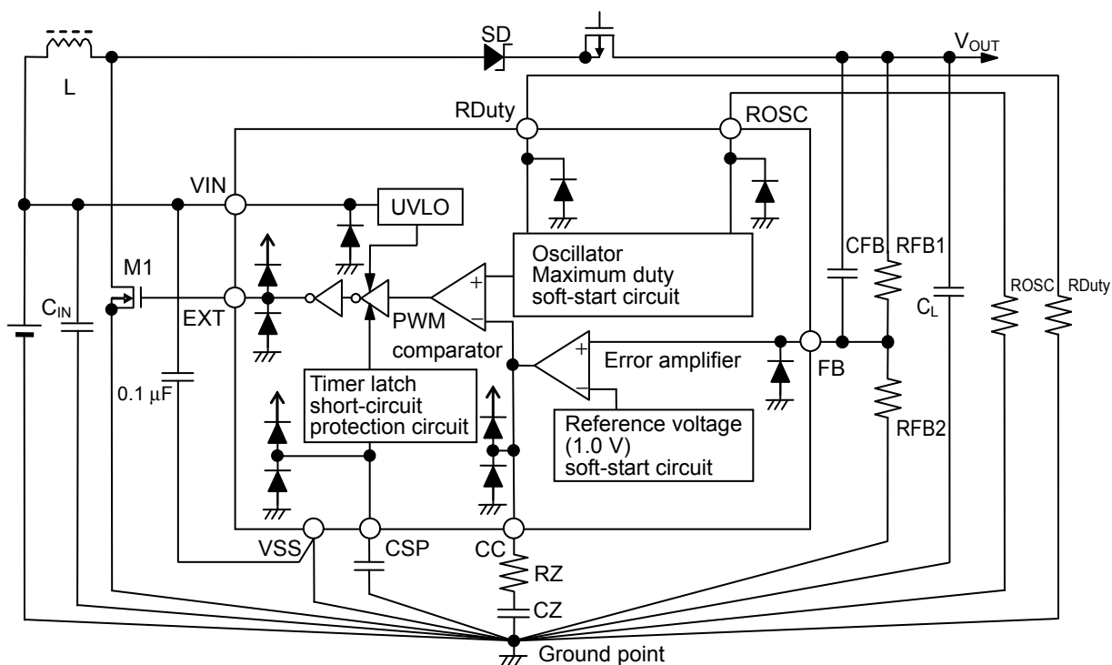
Figure 15 Standard Circuit
