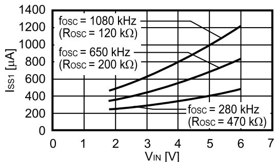
I_{SS1} vs. V_{IN}
