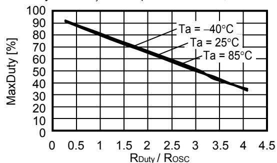
MaxDuty vs. R_{Duty} / R_{osc} ( R_{osc} = 200 kΩ, V_{IN} = 3.3 V)
