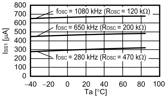
I_{SS1} vs. T_a ( V_{IN} = 3.3\text{ V} )
