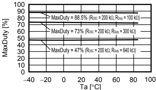
MaxDuty vs. T_a ( V_{IN} = 3.3\text{ V} )
