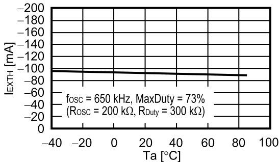
I_{EXTH} vs. T_a ( V_{IN} = 3.3\text{ V} )
