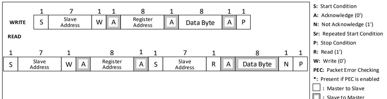
Figure 24: I2C Format
