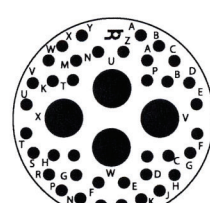
25-42 - 25-42*• 38 #20, 4 #8 Coax I, Coax Service Ratings I
