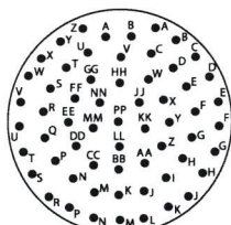
25-61 24-61† 25-61 61 #20 Service Ratings I
