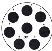
25-8 - 25-8*• 8 #8 Twinax Service Ratings Twinax
