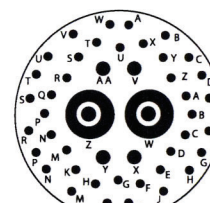
25-46 - 25-46 40 #20, 4 #16, 2 #8 Twinax Service Ratings Twinax
