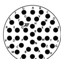
25-37 - 25-37*• 37 #16 Service Ratings II I
