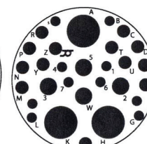
25-20 - 25-20*• 3 #8 Twinax, 13 #16, 4 #12 Coax, 10 #20 N / Coax / Twinax Service Ratings I
