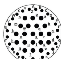
25-43 - 25-43 23 #20, 20 #16 Service Ratings I
