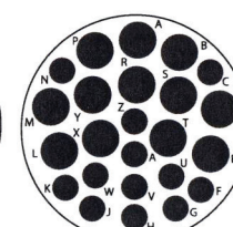
25-24 24-24† 25-24 12 #16, 12 #12 Service Ratings I
