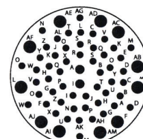
25-66*• - 25-66*• 53 #22D, 2 #20, 11 #16 Service Ratings I
