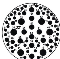
25-64 - 25-64 40 #22D, 8 #20 10 #16, 6 #12 Service Ratings I
