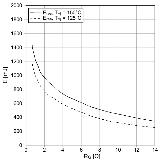
Schaltverluste Diode-Brems-Chopper switching losses Diode-brake-chopper E_{rec} = f(R_G) I_F = 1000 A , V_{CE} = 1800 V
