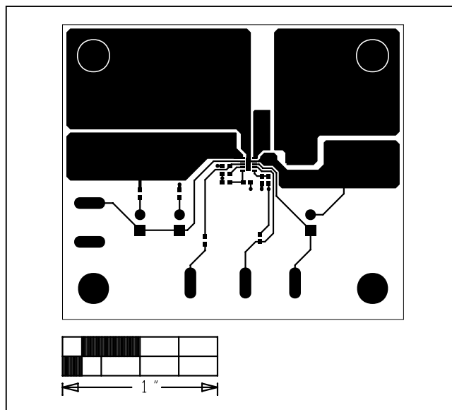
Figure 2. MAX17532 5V EV Kit (TDFN) PCB Layout—Component Side
