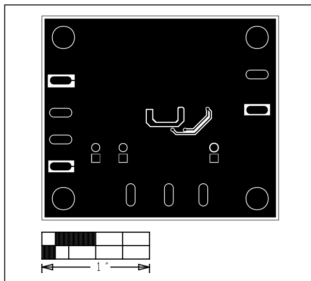
Figure 3. MAX17532 5V EV Kit (TDFN) PCB Layout—Solder Side
