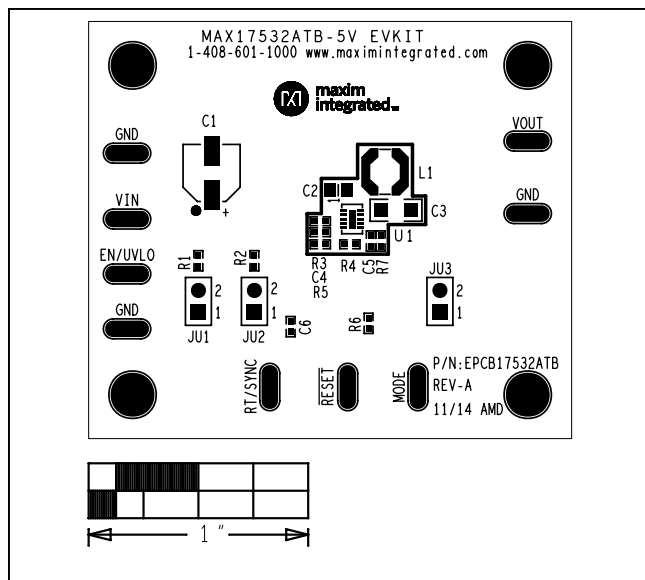
Figure 1. MAX17532 5V EV Kit (TDFN) Component Placement Guide—Component Side
