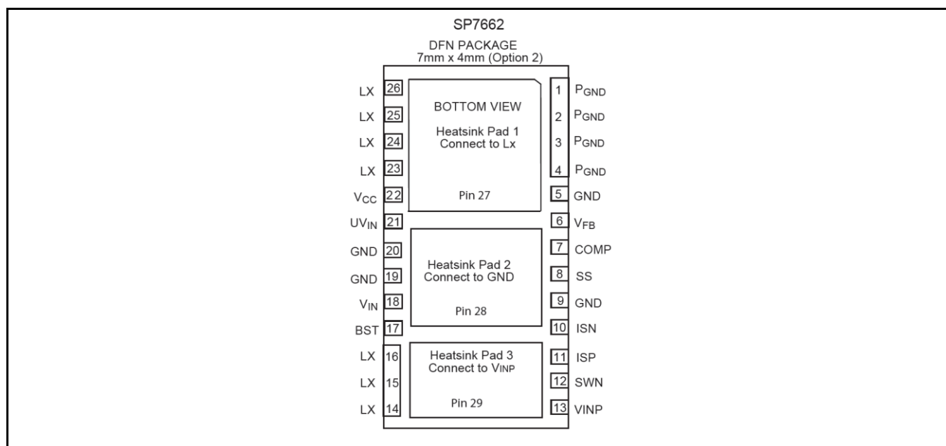
PIN ASSIGNMENT
