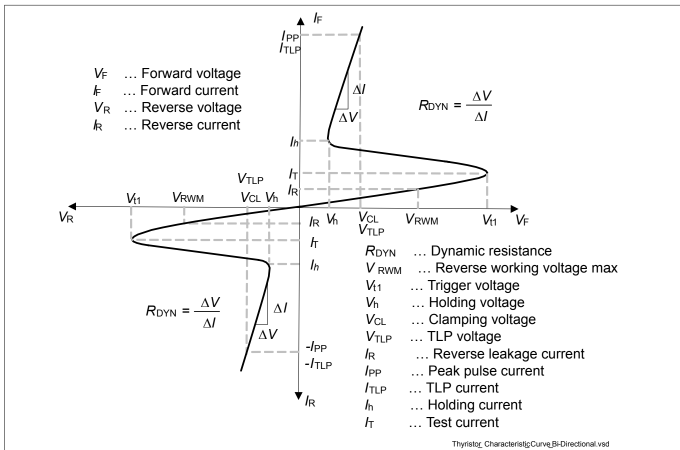
Figure 2 Definitions of electrical characteristics
