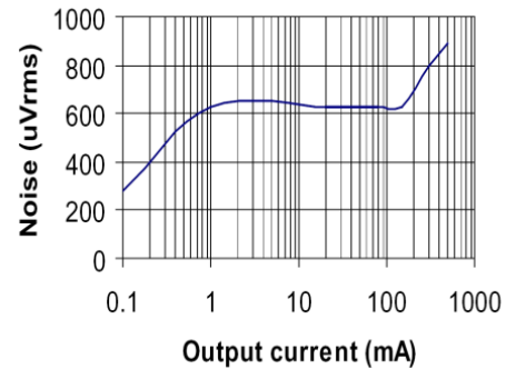
Fig. 20: Output Noise, C_{BYP} = open
