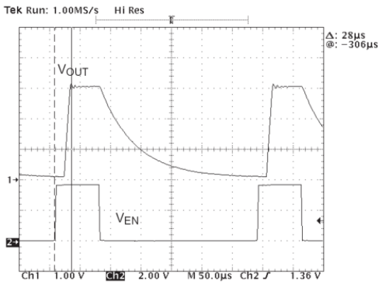
Fig. 6: Turn-Off Time, R_{LOAD}=6\Omega (500mA)
