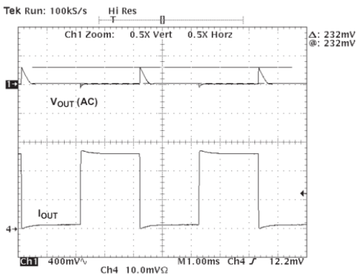
Fig. 8: Load Regulation, I_o=100\mu A \sim 500mA
