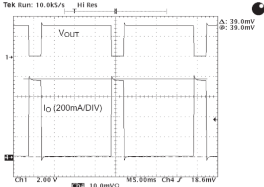
Fig. 4: Current Limit
