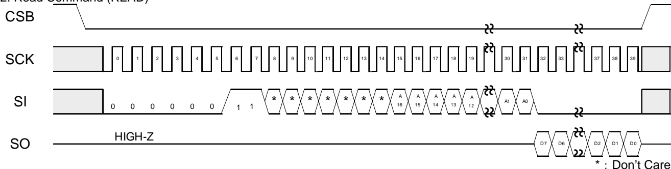
Figure 39. Read command
