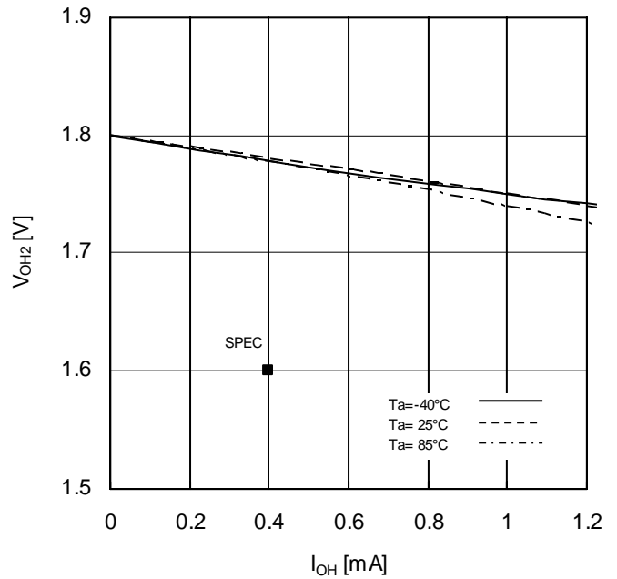
Figure 10. Output High Voltage2 vs Output Current (Vcc=1.8V)
