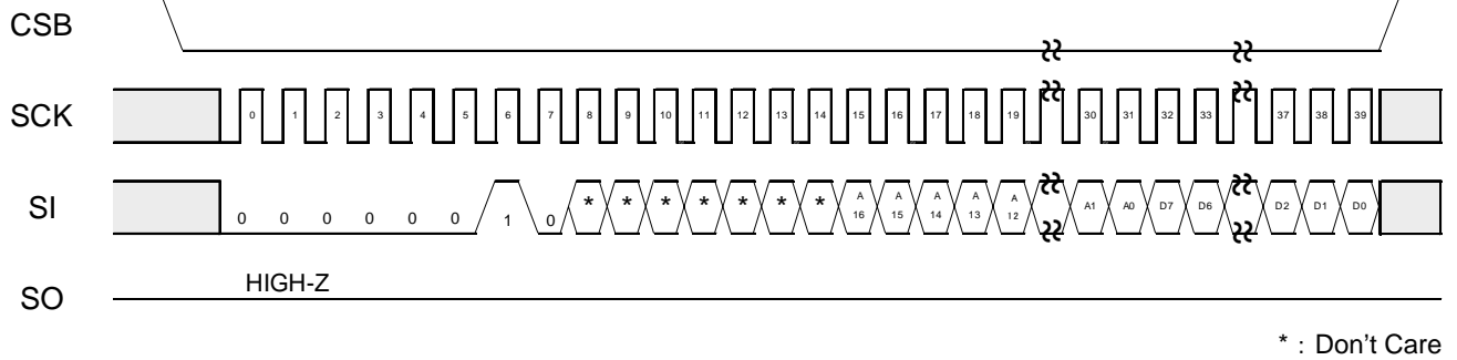
Figure 40. Write command
