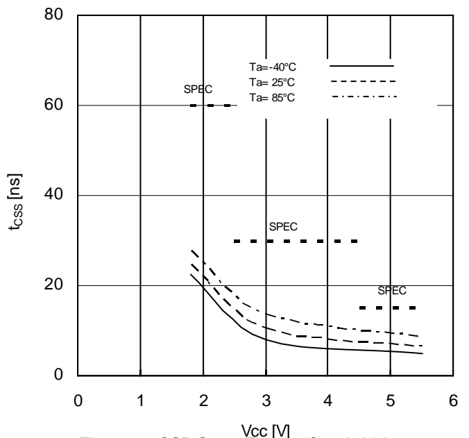
Figure 24. CSB Setup Time vs Supply Voltage
