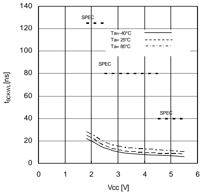
Figure 22. SCK Low Time vs Supply Voltage
