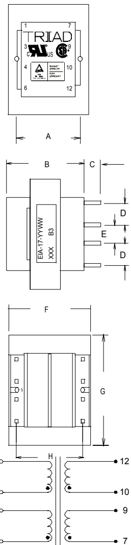
SCHMATIC
