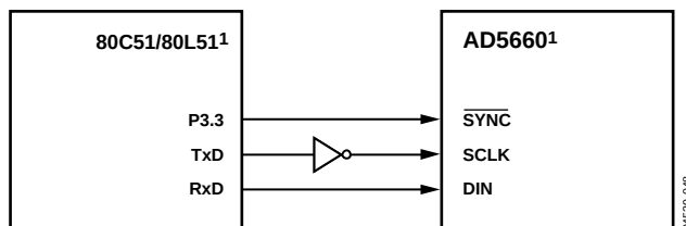
Figure 47. AD5660-to-80C51/80L51 Interface
