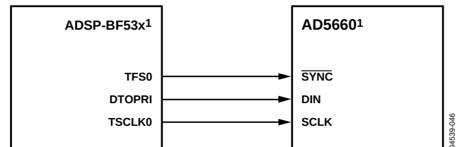
Figure 45. AD5660-to-Blackfin ADSP-BF53x Interface
