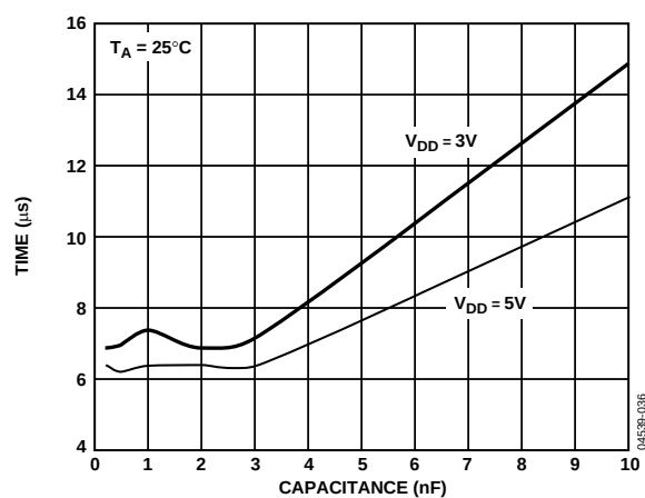
Figure 34. Settling Time vs. Capacitive Load
