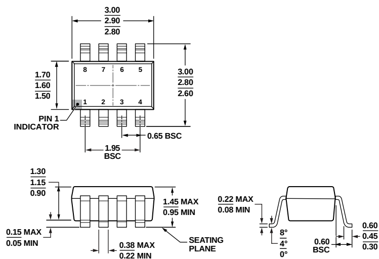
Figure 53. 8-Lead Small Outline Transistor Package [SOT-23] (RJ-8) Dimensions shown in millimeters
