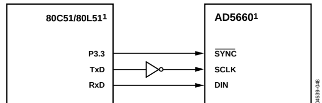
Figure 47. AD5660-to-80C51/80L51 Interface
