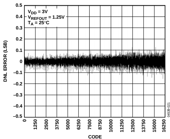
Figure 15. DNL—AD5640-1
