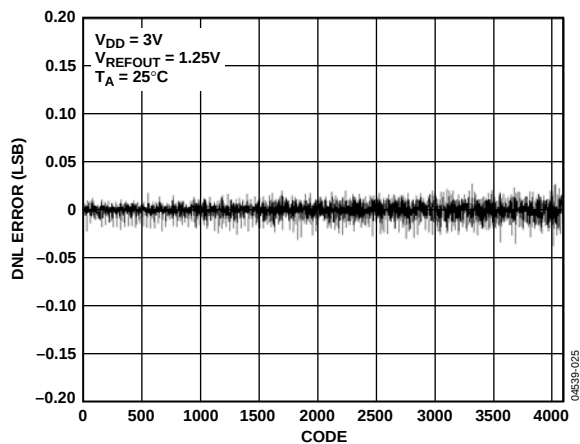
Figure 16. DNL—AD5620-1
