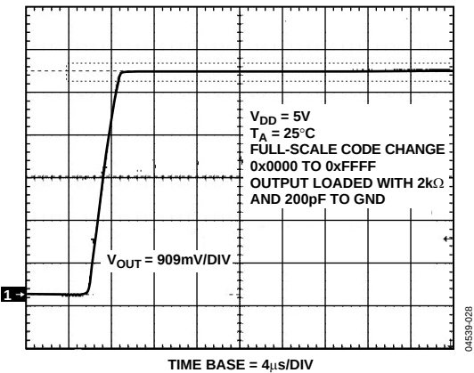
Figure 26. Full-Scale Settling Time, 5 V
