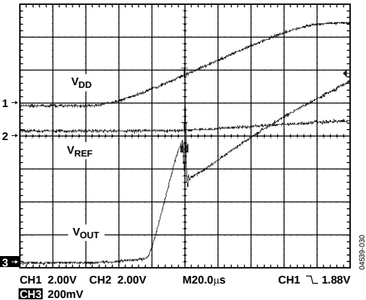
Figure 28. Power-On Reset to Midscale—AD5660-3
