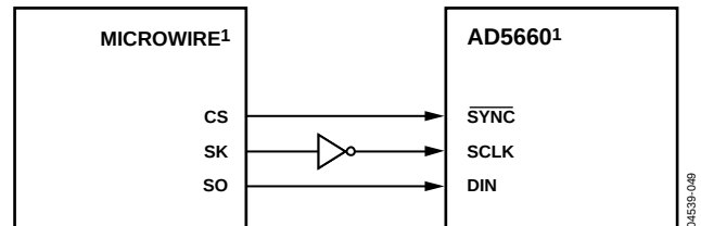
Figure 48. AD5660-to-MICROWIRE Interface
