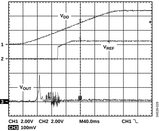
Figure 27. Power-On Reset to 0 V—AD5660-2
