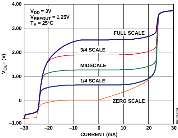
Figure 23. Source and Sink Capability—AD5660-1
