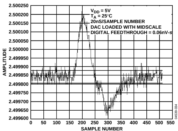
Figure 33. Digital Feedthrough
