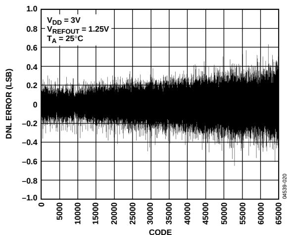
Figure 14. DNL—AD5660-1
