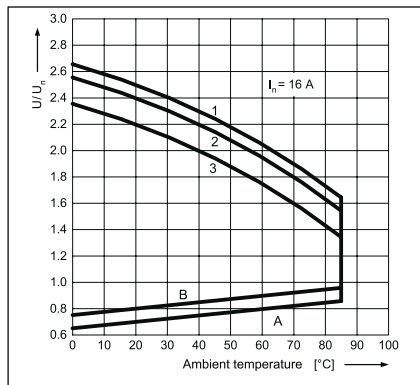
Coil operating range - DC Fig. 4.2
