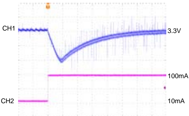
200 \mu sec/div CH1: V_{out1} , AC-COUPLED, 50mV/div CH2: I_{out1} , 50mA/div
