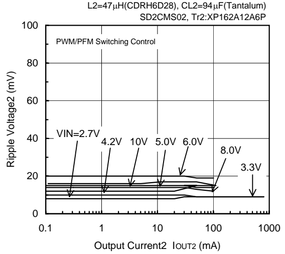
FOSC=180kHz, VOUT2=1.0V
