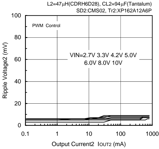
FOSC=180kHz, VOUT2=3.3V
