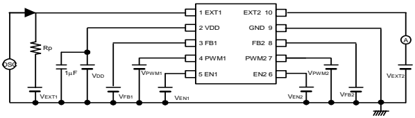
Circuit 7
