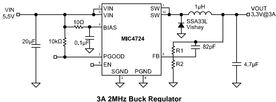
3A 2MHz Buck Regulator
