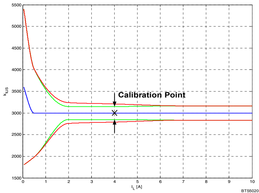
Figure 22 Improved SENSE Accuracy with One Calibration Point
