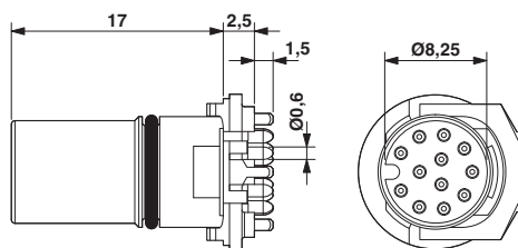
M12 socket, straight
