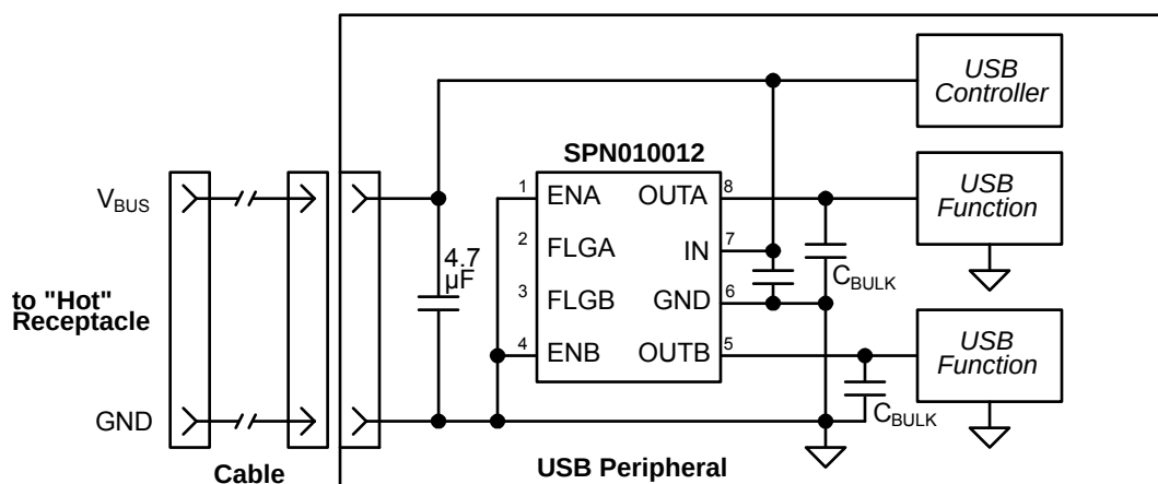
Figure 3. Hot-Plug Application
