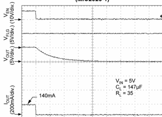
Turn-Off (MIC2026-1)
