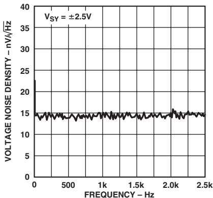
TPC 41. Voltage Noise Density
