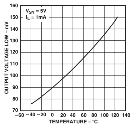
TPC 45. Output Voltage Low vs. Temperature
