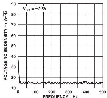
TPC 39. Voltage Noise Density
