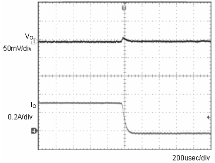
Fig.4 Transient Response (0.3→0A) Co=1μF
