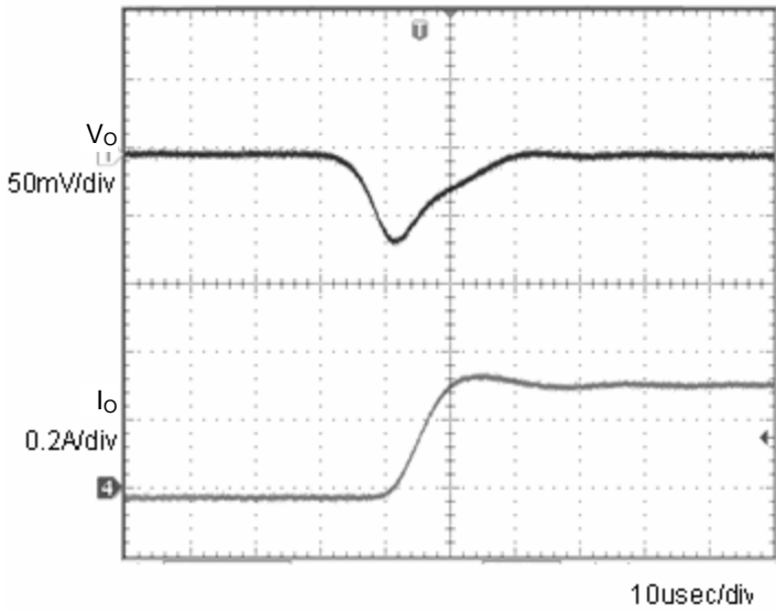
Fig.3 Transient Response (0→0.3A) Co=1μF
