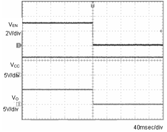
Fig.8 OFF sequence 2 C_o=1\mu F
