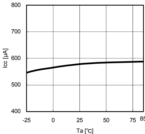
Fig.8 Ta-Icc
