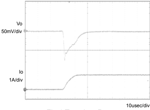
Fig.1 Transient Response (0→1.5A) Co=1 µF
