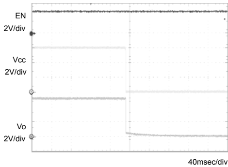
Fig.4 OFF sequence 1 Co=1 µF
