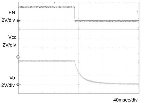
Fig.6 OFF sequence 2 Co=1 µF
