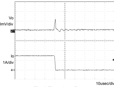
Fig.2 Transient Response (1.5→0A) Co=1 µF
