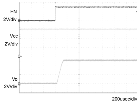
Fig.5 Input sequence 2 Co=1 µF
