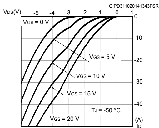
Figure 9. 3 rd quadrant characteristics @ T_J = -50^\circ\text{C}
