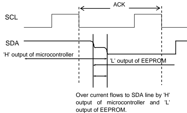
Figure 40. Input / Output Collision Timing
