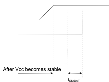
Figure 47. When SCL='L' and SDA='L'
