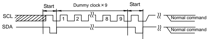
Figure 34.-(b) The case of START + dummy clock \times 9 + START + command input
