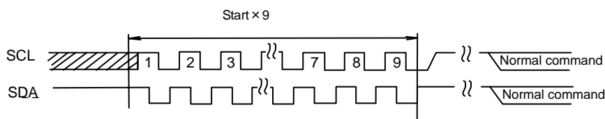
Figure 34.-(c) START \times 9 + command input
