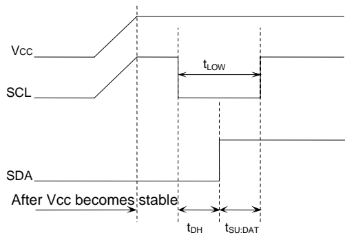
Figure 46. When SCL='H' and SDA='L'
