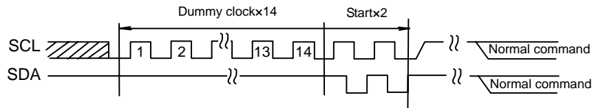
Figure 34.-(a) The case of dummy clock \times 14 + START+START+ command input
