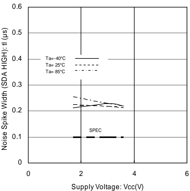
Figure 25. Noise Spike Width vs Supply Voltage (SDA H)
