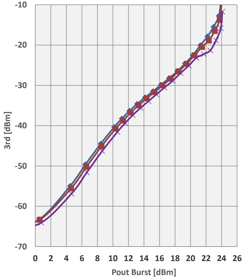
3rd Harmonic
