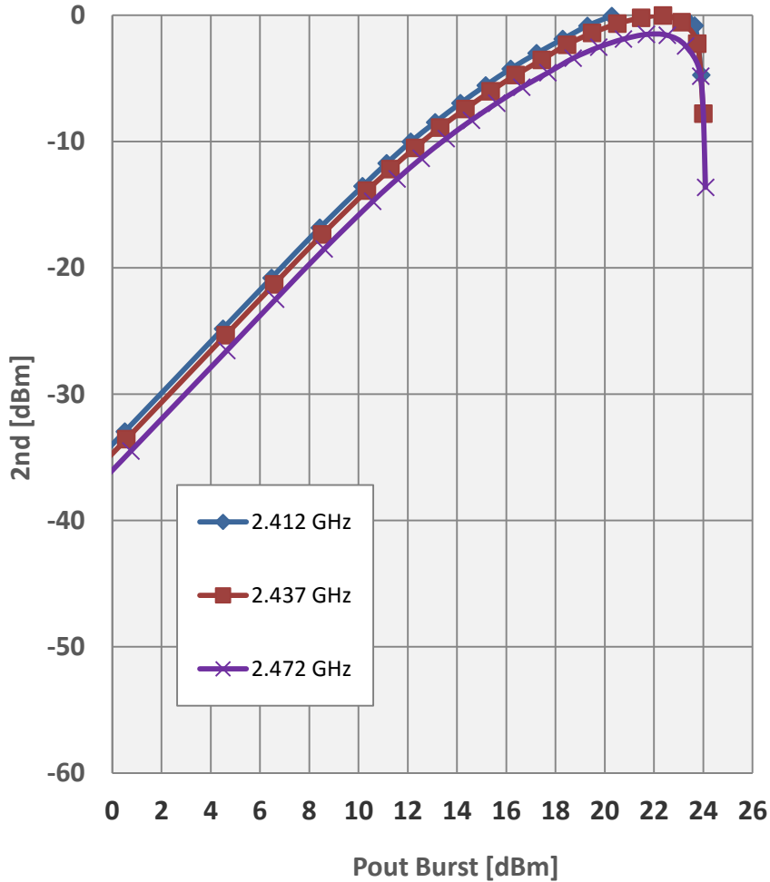
2nd Harmonic
