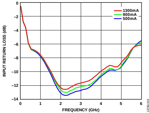
Figure 16. Input Return Loss vs. Frequency at Various Quiescent Supply Currents ( I_{DDX} )
