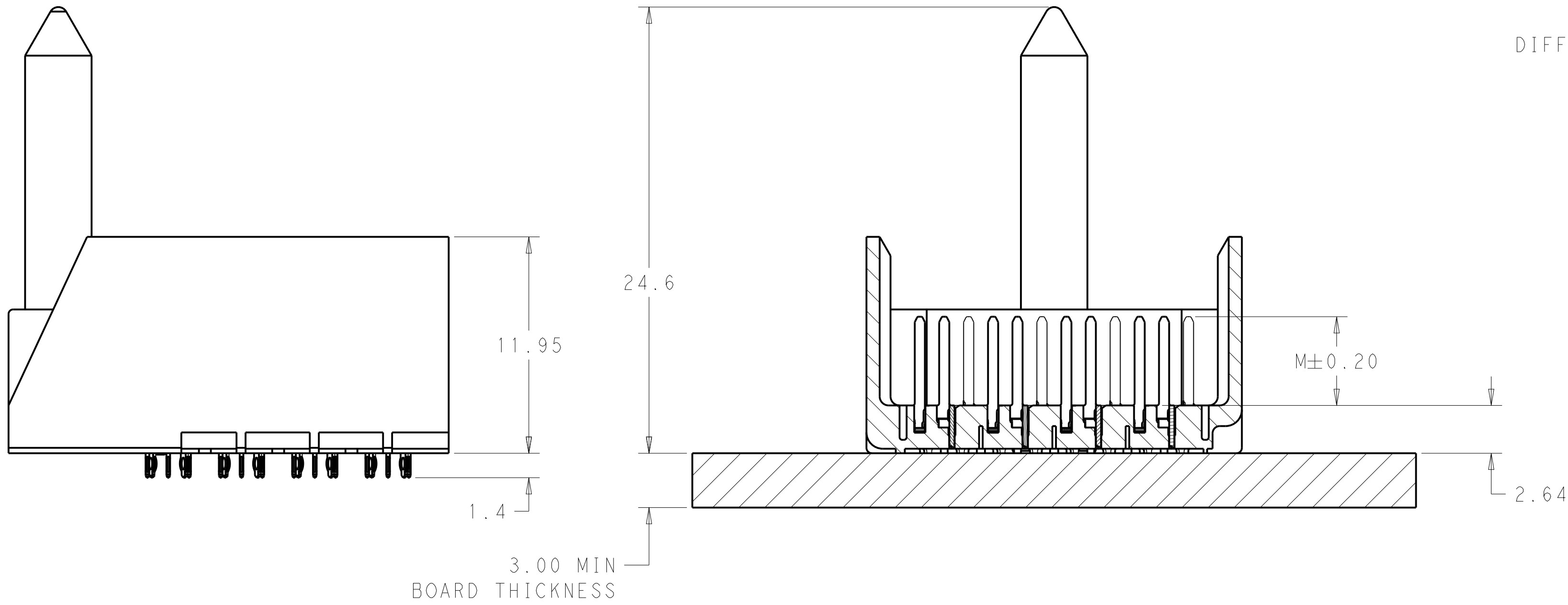
SECTION Z-Z
