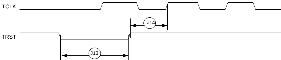
Figure 26. \overline{\text{TRST}} Timing
