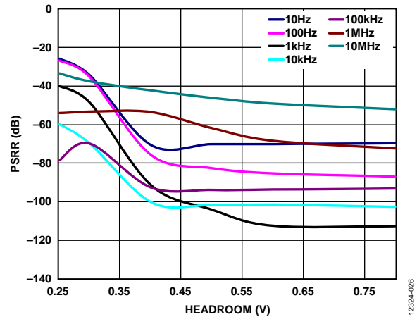
Figure 26. Power Supply Rejection Ratio (PSRR) vs. Headroom Voltage, Different Frequencies, V_{OUT} = 1.8\text{ V} , 400 mA Load
