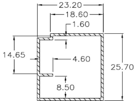
Profile view
