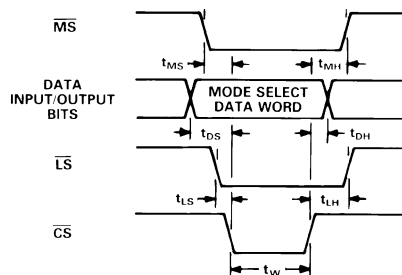
Figure 17a. Preload Mode Select Register
