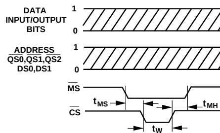
Figure 17c. Update Second Rank of Mode Select Latch
