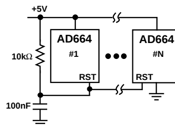
Figure 24. Power-On Reset
