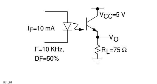
Figure 1. Non-saturated Switching Schematic
