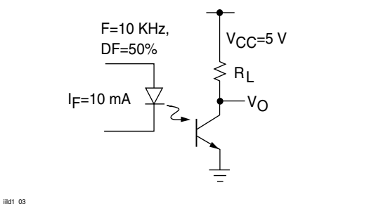
Figure 3. Saturated Switching Schematic
