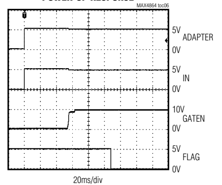
POWER-UP RESPONSE
