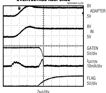
OVERVOLTAGE RESPONSE
