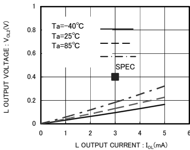
Fig.6 'L' output voltage V_{OL2} \sim OL_n ( V_{CC}=2.5V )
